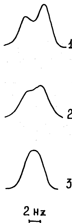
Figure 1. The lineshapes of COOCH_3 signals of enamine 1 with R = H in pyridine at 70^\circ C and various concentrations (1.0 - 0.1 M, 2.0 - 0.3 M, 3.0 - 0.4 M).
